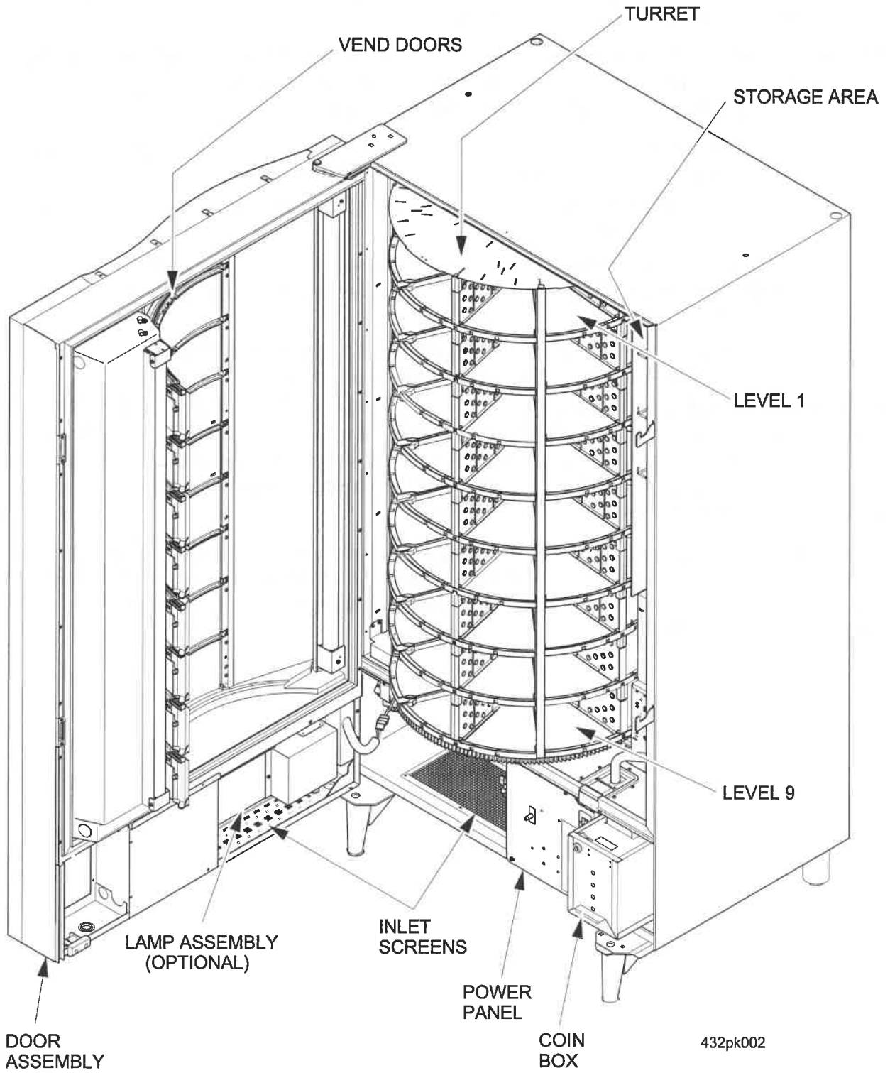
FIGURE 1: 432/962 MERCHANDISER
